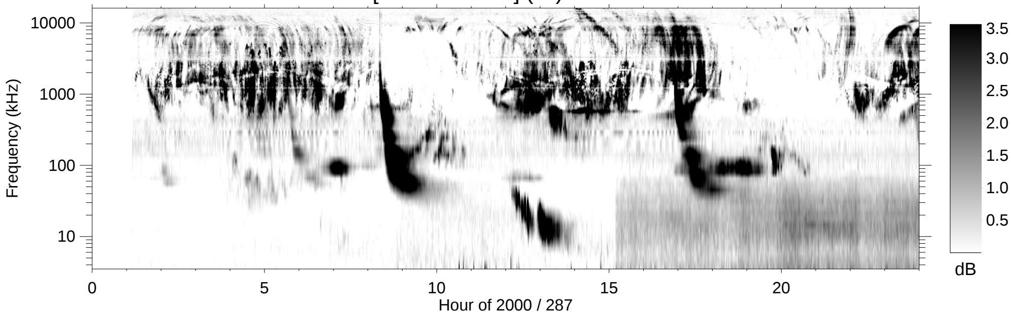
RPWS [ABCH1H2/Ex] (-B) 2000/10/13
