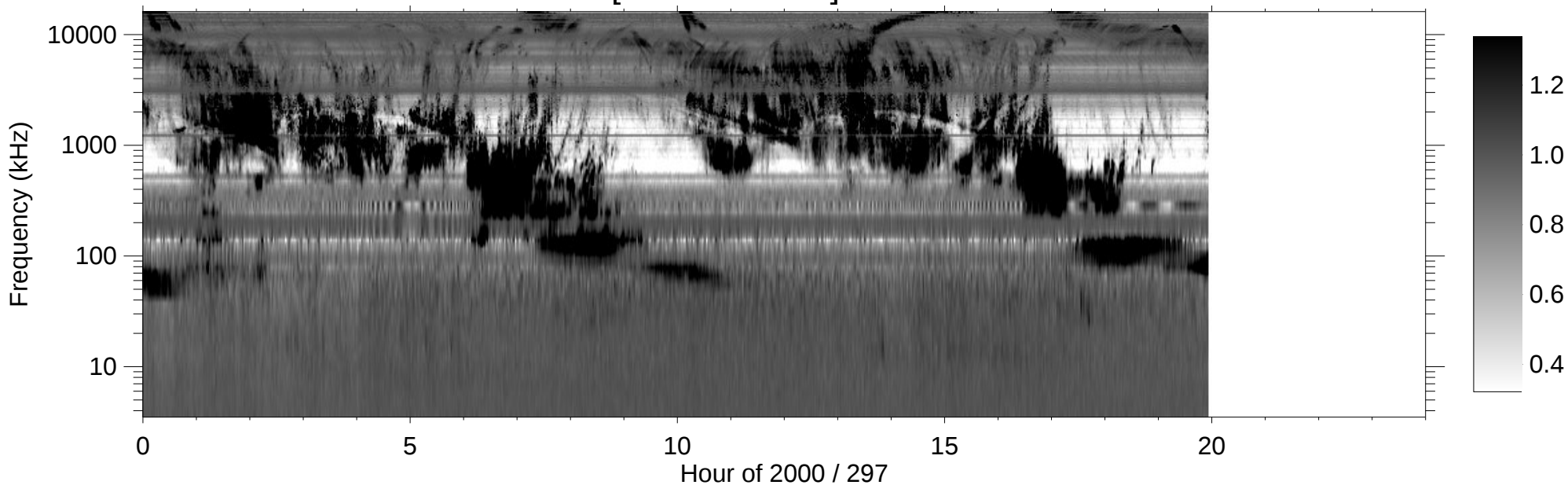
RPWS [ABCH1H2/Ex] (-B) 2000/10/23
