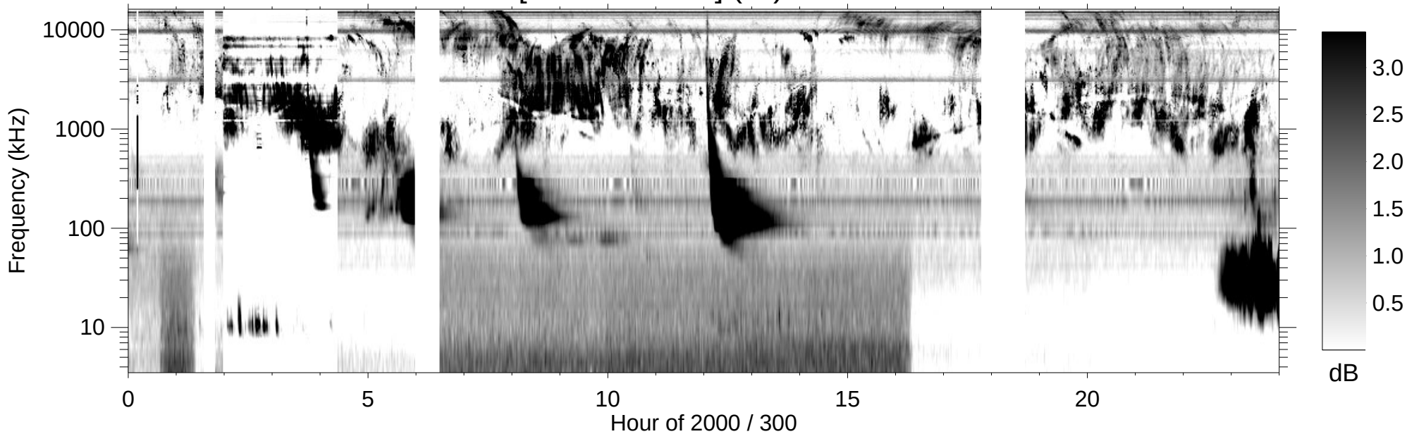
RPWS [ABCH1H2/Ex] (-B) 2000/10/26
