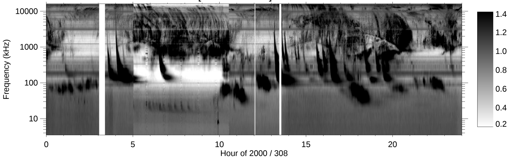
RPWS [ABCH1H2/Ex] (-B) 2000/11/03
