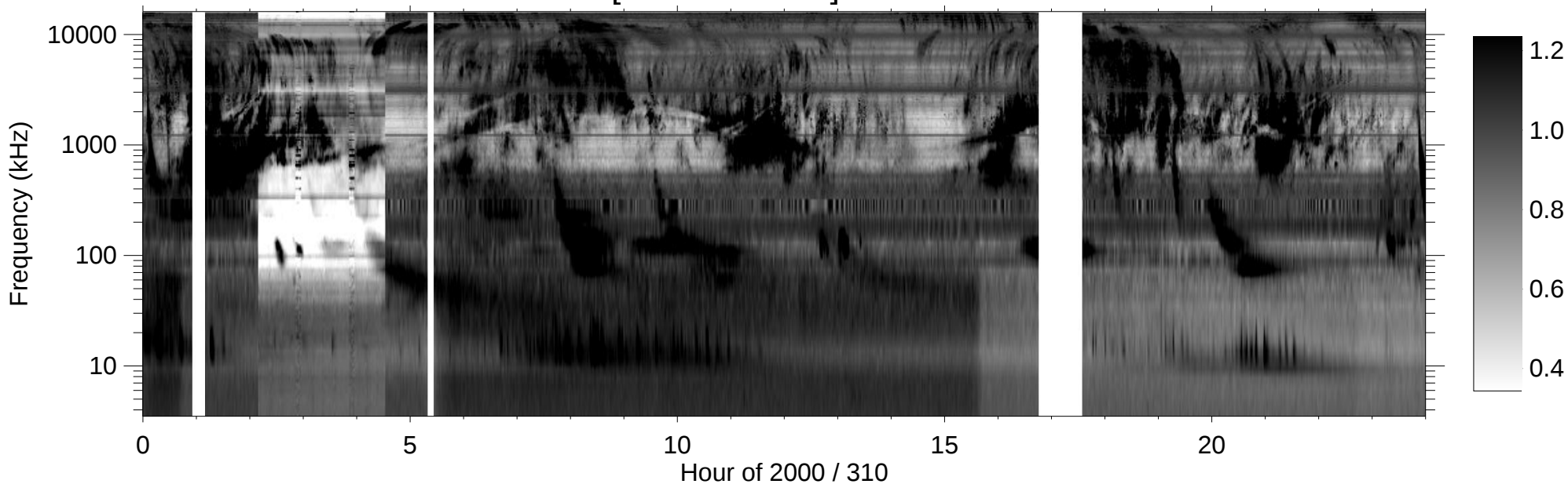
RPWS [ABCH1H2/Ex] (-B) 2000/11/05
