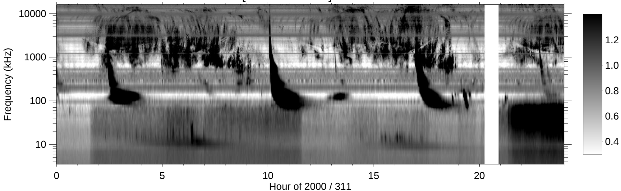
RPWS [ABCH1H2/Ex] (-B) 2000/11/06
