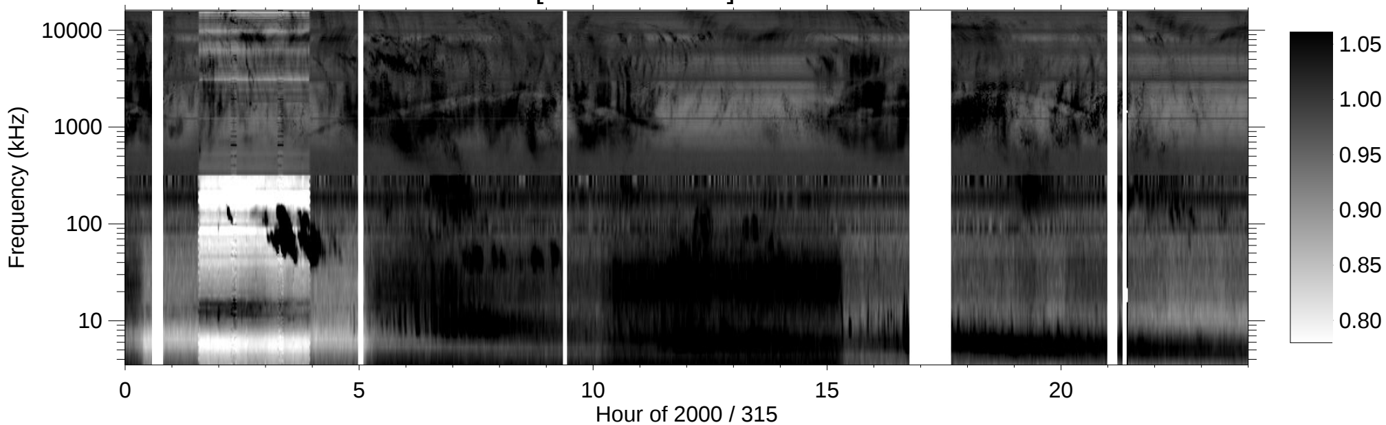
RPWS [ABCH1H2/Ex] (-B) 2000/11/10
