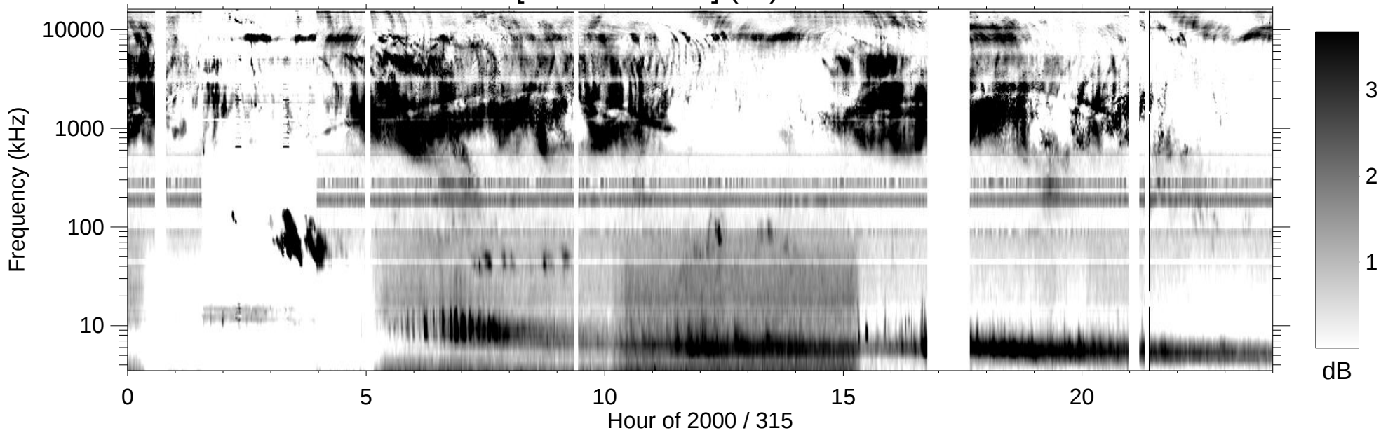
RPWS [ABCH1H2/Ex] (-B) 2000/11/10
