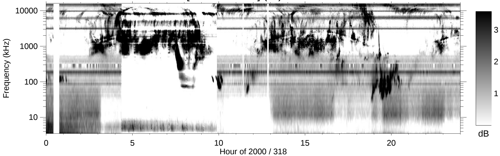
RPWS [ABCH1H2/Ex] (-B) 2000/11/13
