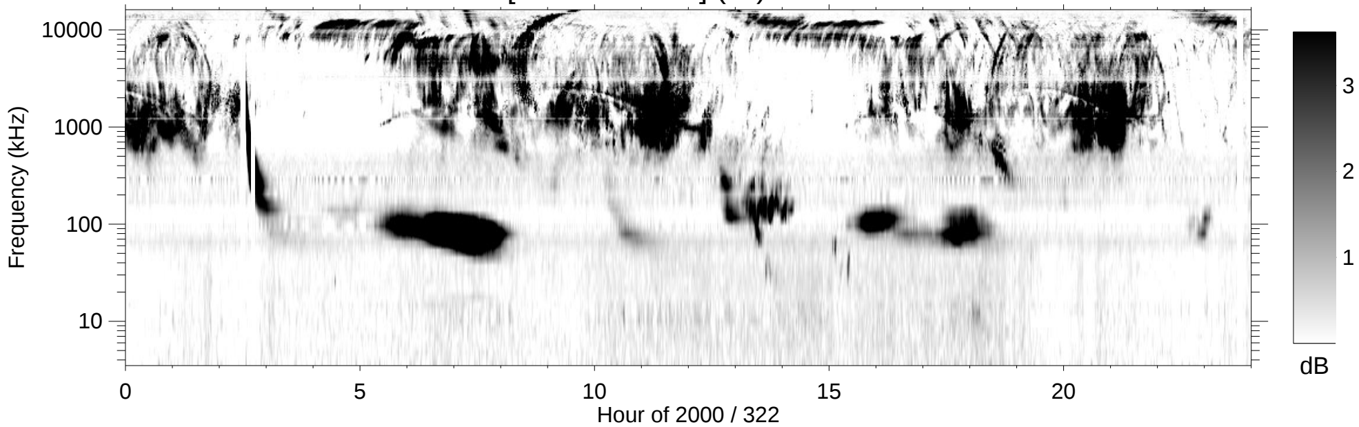
RPWS [ABCH1H2/Ex] (-B) 2000/11/17
