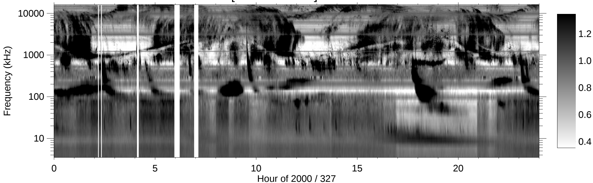
RPWS [ABCH1H2/Ex] (-B) 2000/11/22
