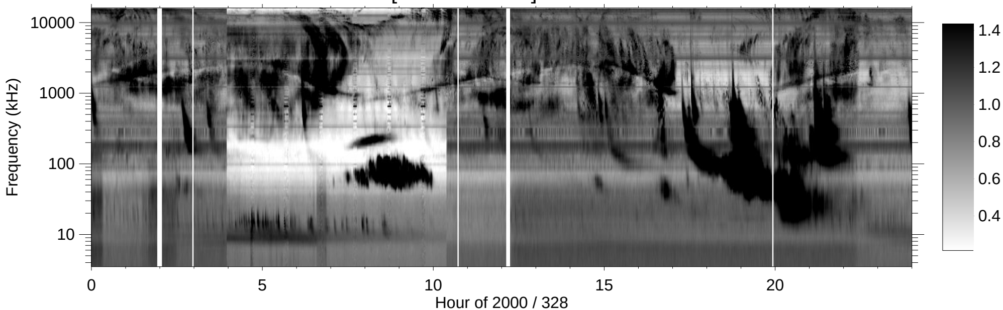
RPWS [ABCH1H2/Ex] (-B) 2000/11/23
