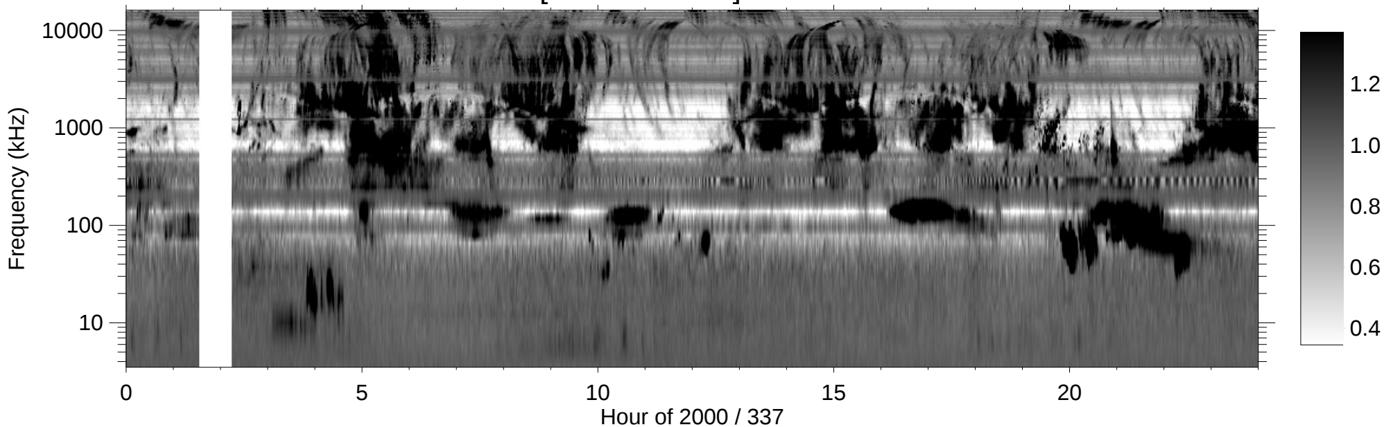
RPWS [ABCH1H2/Ex] (-B) 2000/12/02
