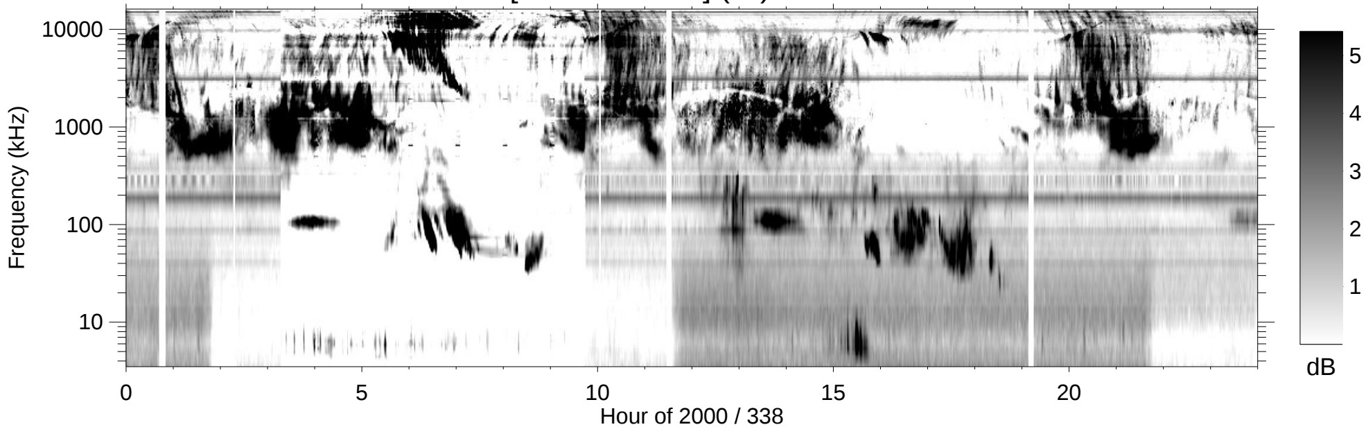
RPWS [ABCH1H2/Ex] (-B) 2000/12/03
