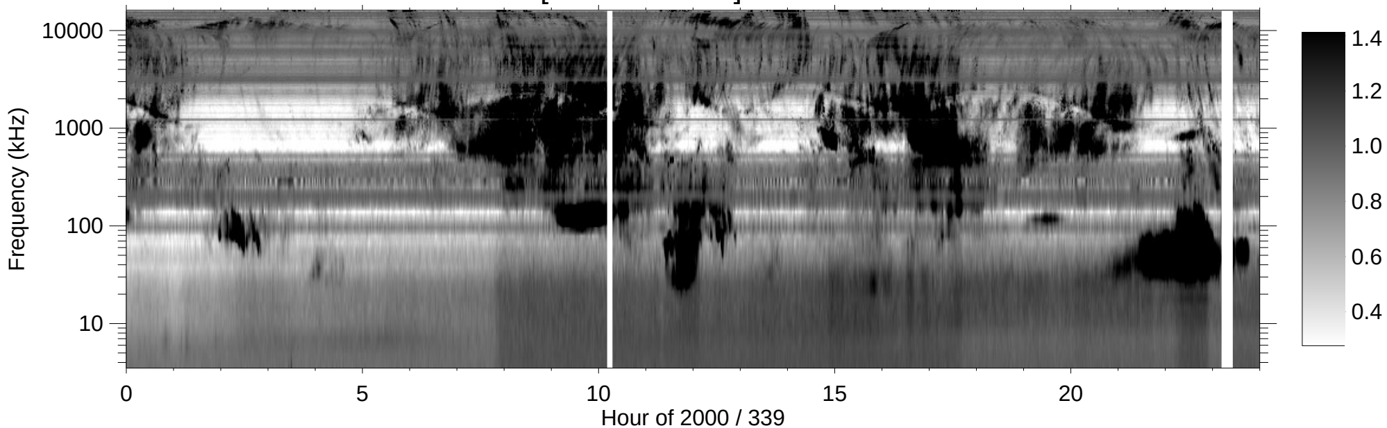
RPWS [ABCH1H2/Ex] (-B) 2000/12/04
