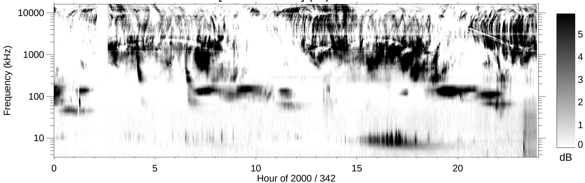
RPWS [ABCH1H2/Ex] (-B) 2000/12/07
