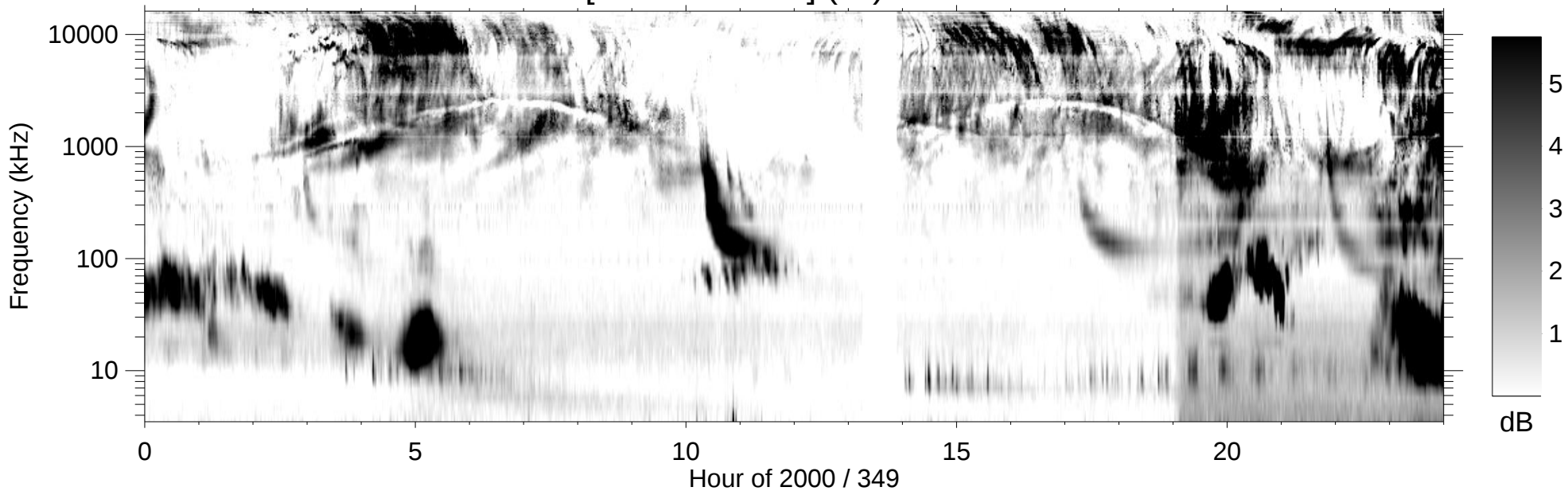
RPWS [ABCH1H2/Ex] (-B) 2000/12/14
