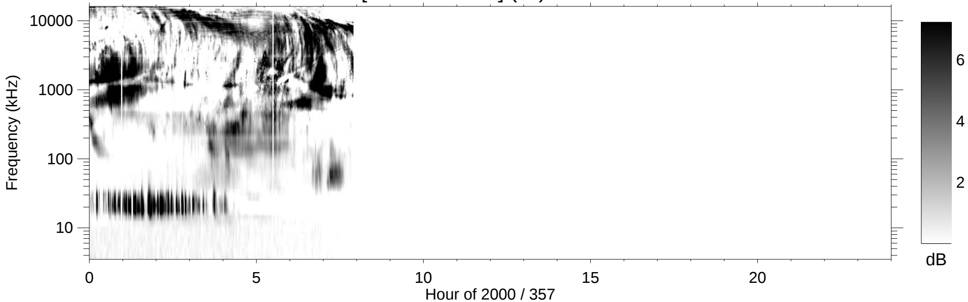
RPWS [ABCH1H2/Ex] (-B) 2000/12/22
