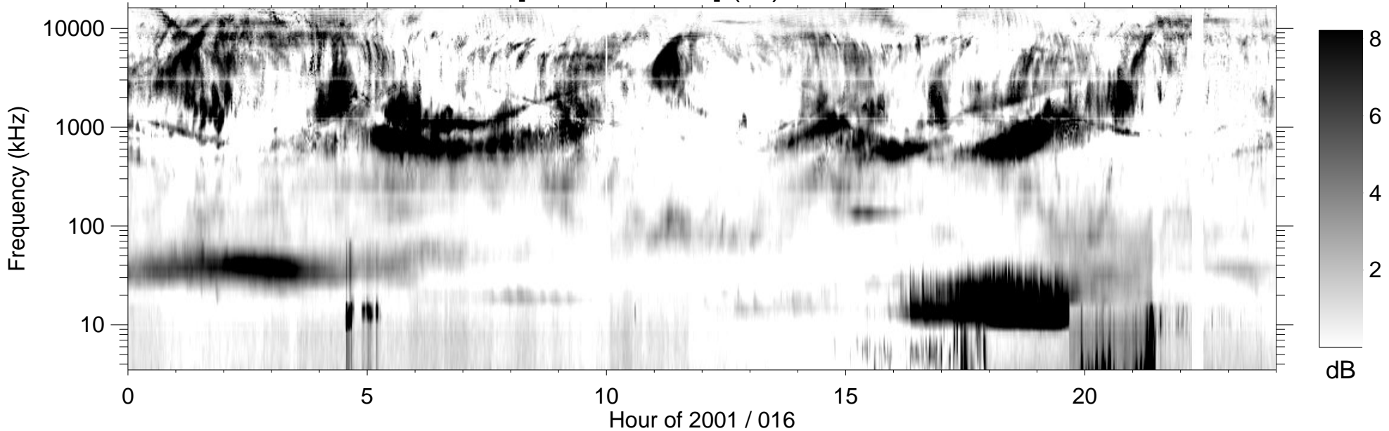
RPWS [ABCH1H2/Ex] (-B) 2001/01/16
