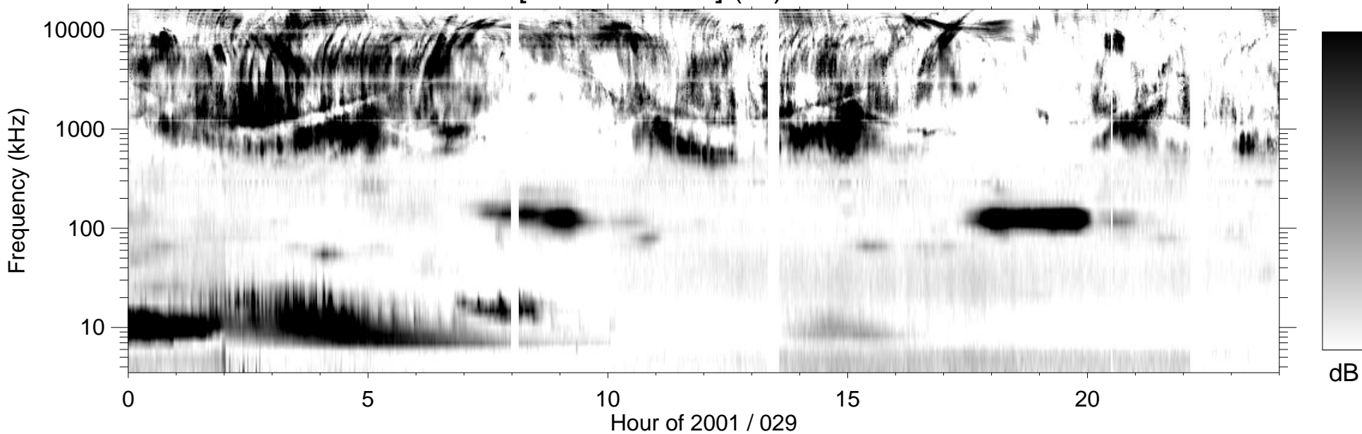
RPWS [ABCH1H2/Ex] (-B) 2001/01/29
