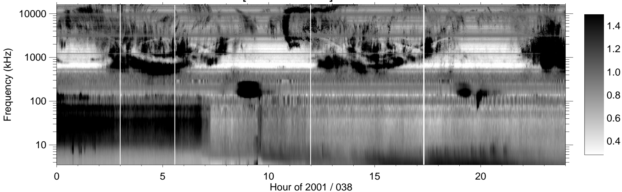
RPWS [ABCH1H2/Ex] (-B) 2001/02/07
