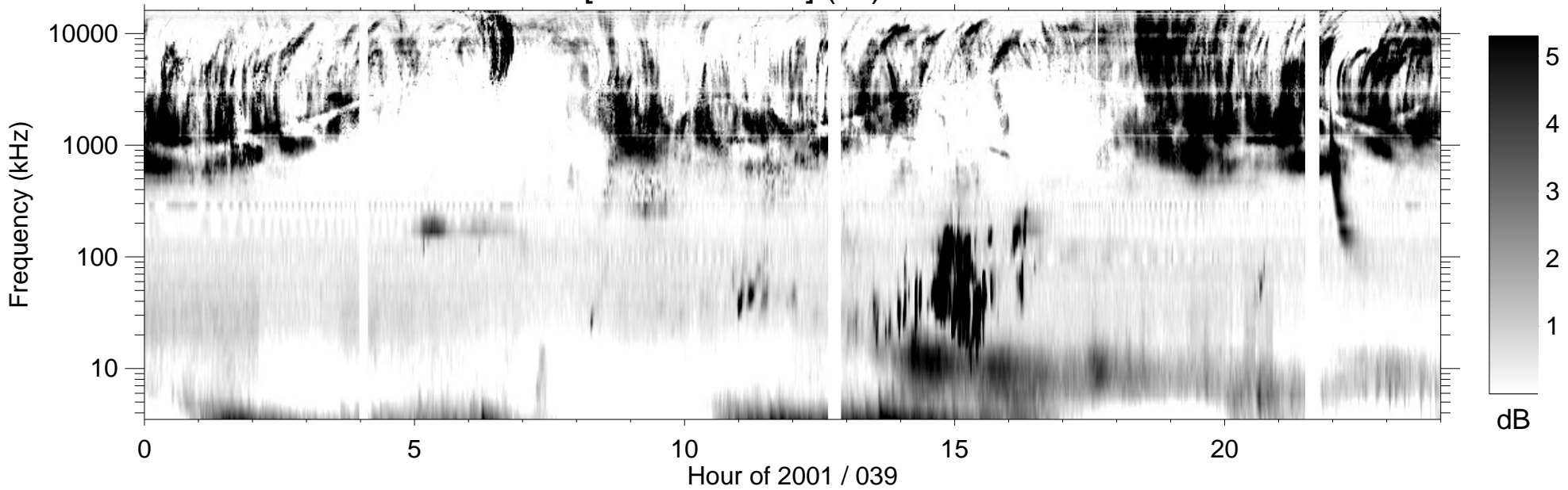
RPWS [ABCH1H2/Ex] (-B) 2001/02/08
