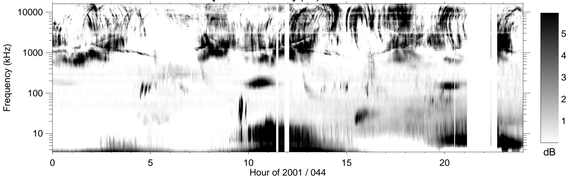
RPWS [ABCH1H2/Ex] (-B) 2001/02/13
