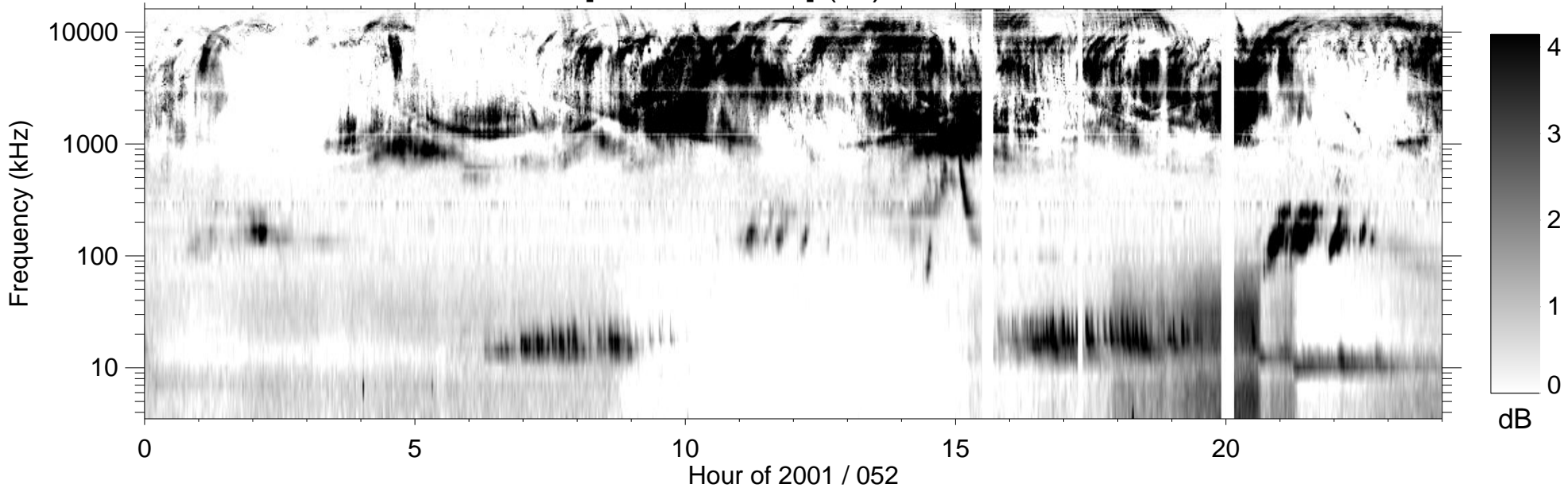
RPWS [ABCH1H2/Ex] (-B) 2001/02/21
