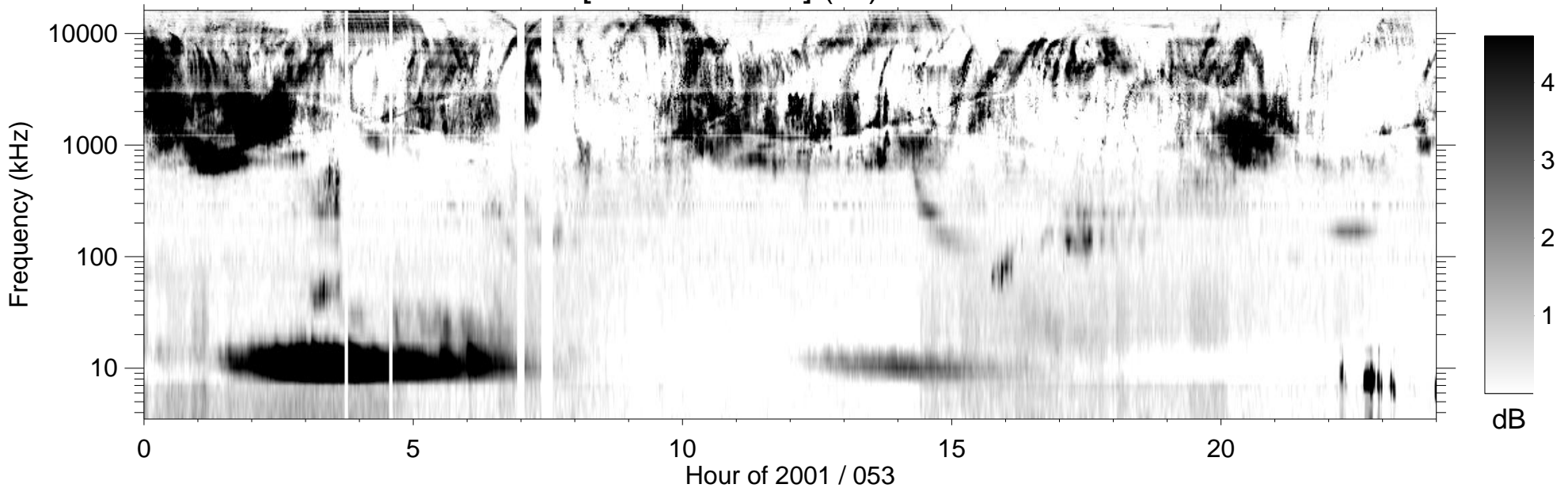
RPWS [ABCH1H2/Ex] (-B) 2001/02/22
