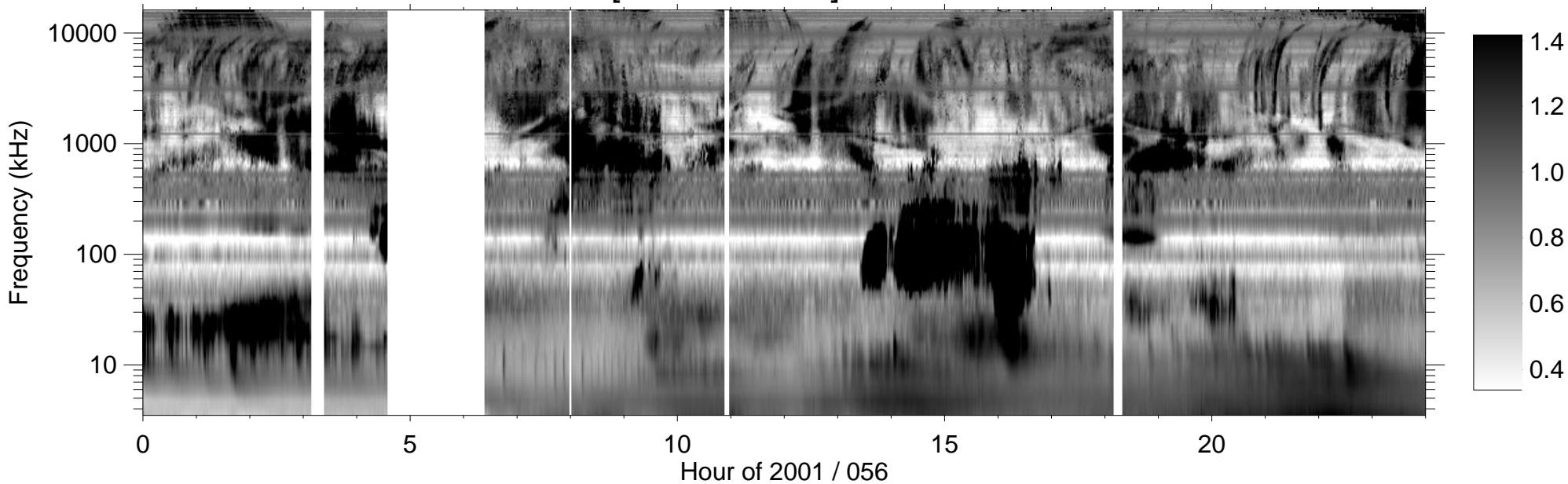
RPWS [ABCH1H2/Ex] (-B) 2001/02/25
