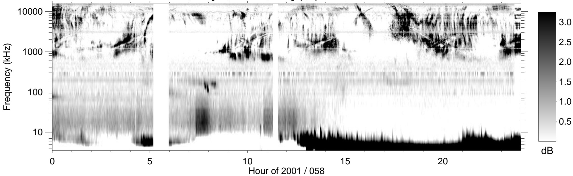
RPWS [ABCH1H2/Ex] (-B) 2001/02/27
