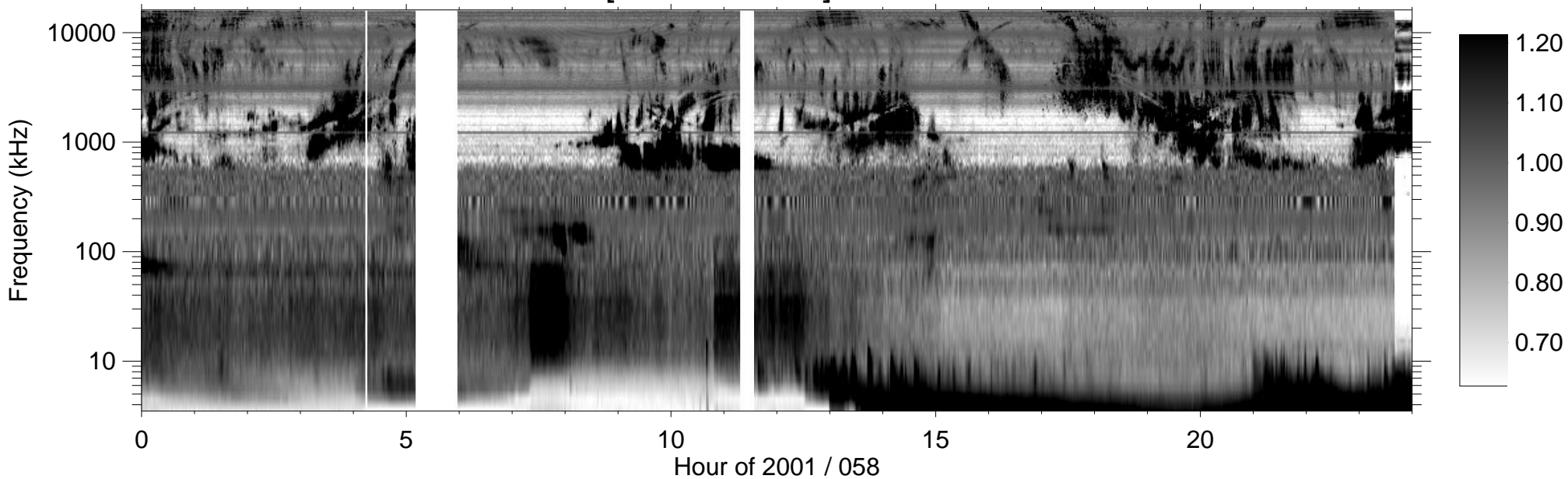
RPWS [ABCH1H2/Ex] (-B) 2001/02/27
