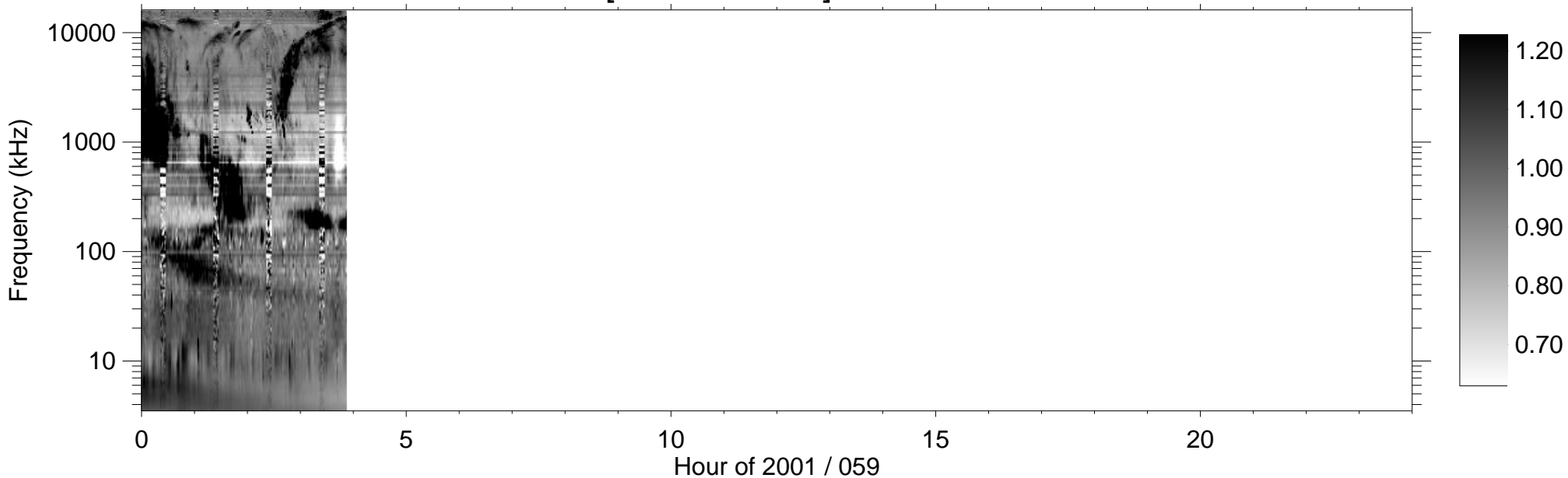
RPWS [ABCH1H2/Ex] (-B) 2001/02/28
