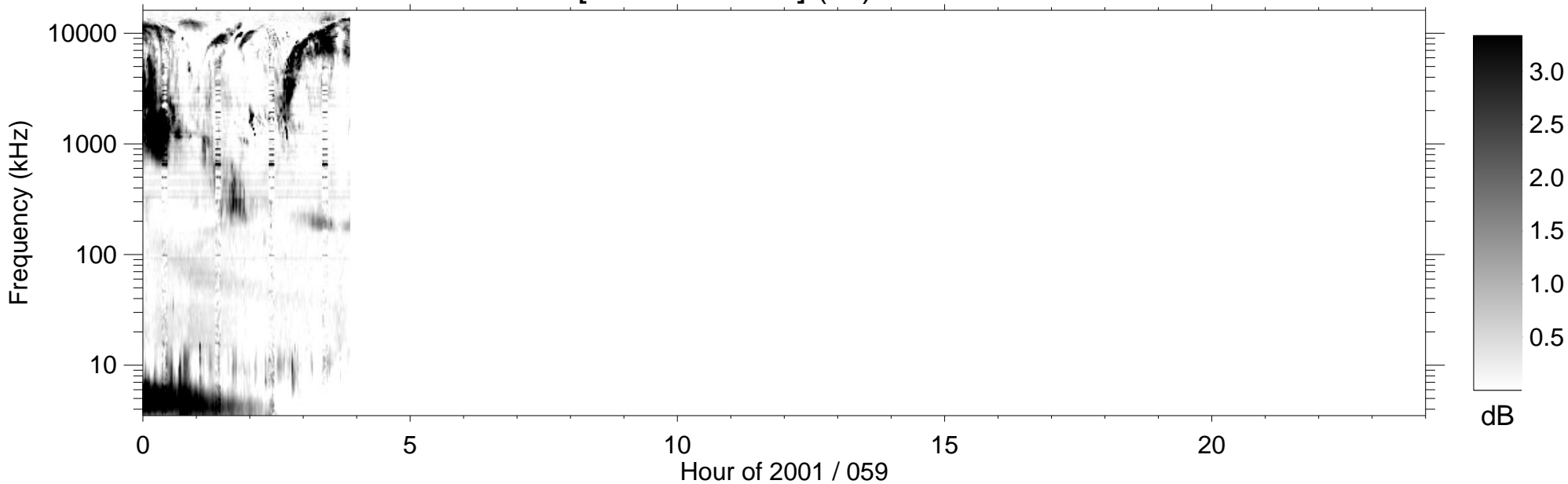
RPWS [ABCH1H2/Ex] (-B) 2001/02/28
