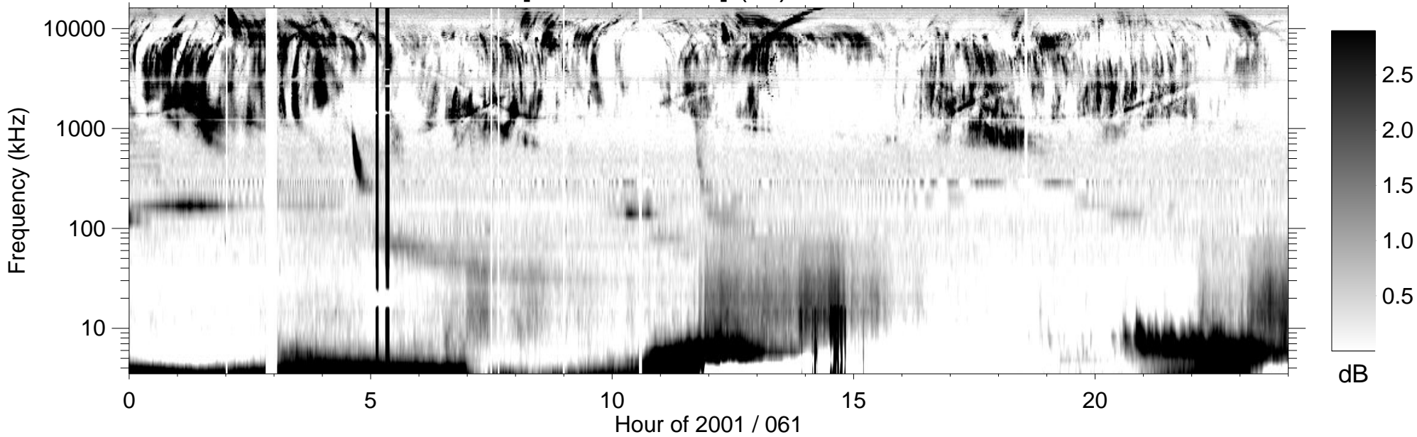
RPWS [ABCH1H2/Ex] (-B) 2001/03/02
