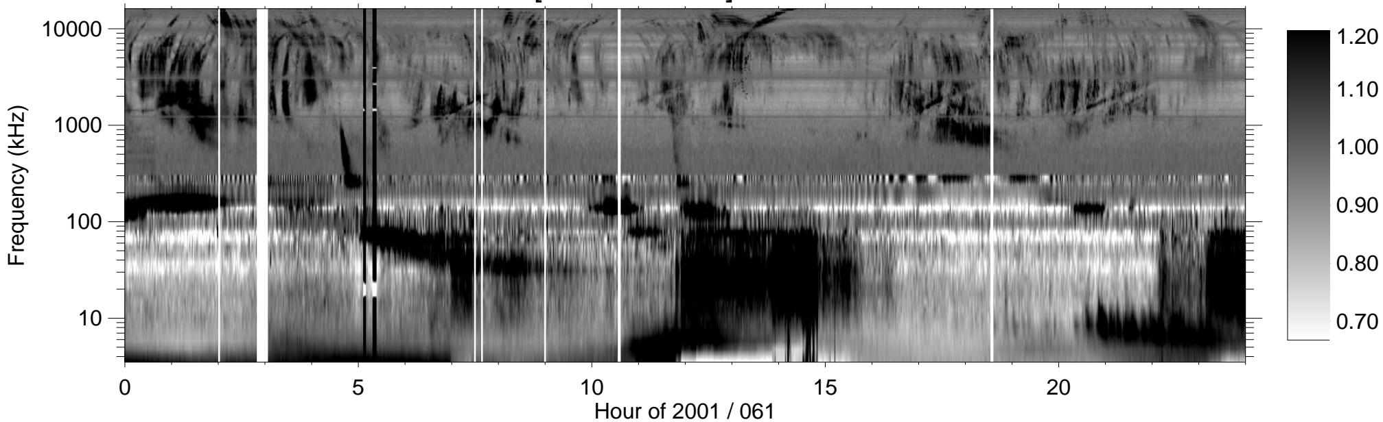
RPWS [ABCH1H2/Ex] (-B) 2001/03/02
