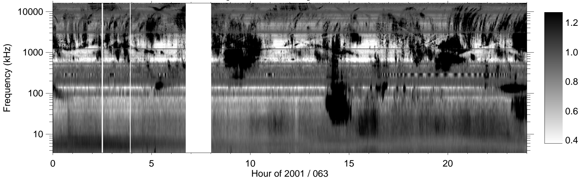
RPWS [ABCH1H2/Ex] (-B) 2001/03/04
