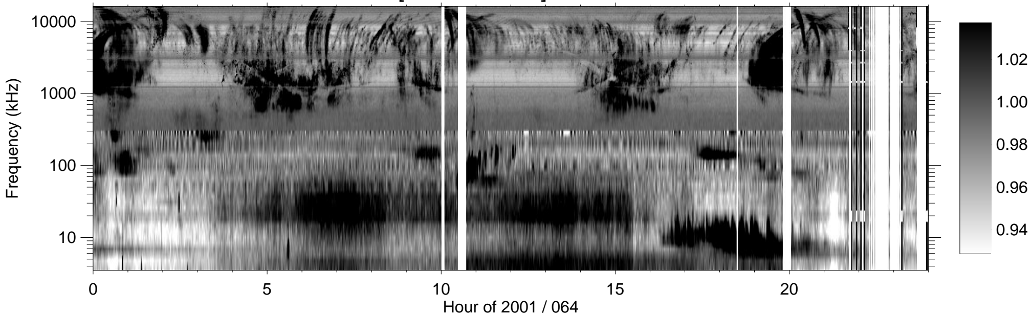
RPWS [ABCH1H2/Ex] (-B) 2001/03/05
