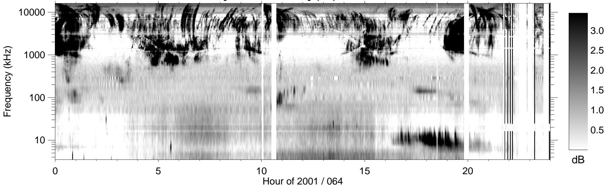
RPWS [ABCH1H2/Ex] (-B) 2001/03/05
