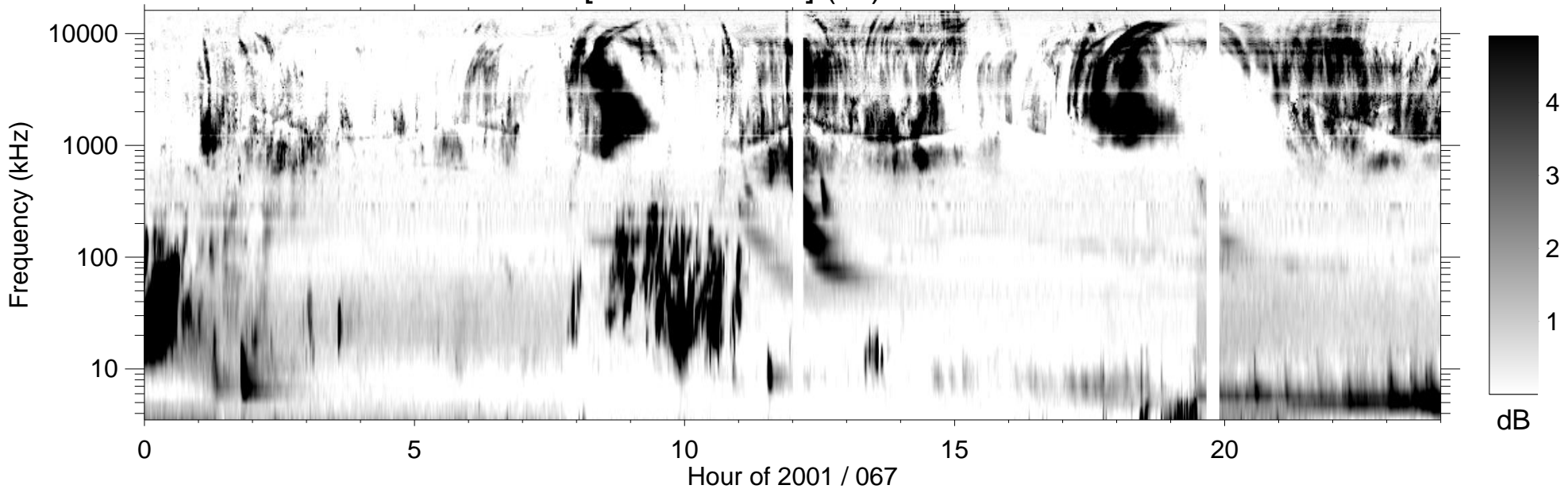
RPWS [ABCH1H2/Ex] (-B) 2001/03/08
