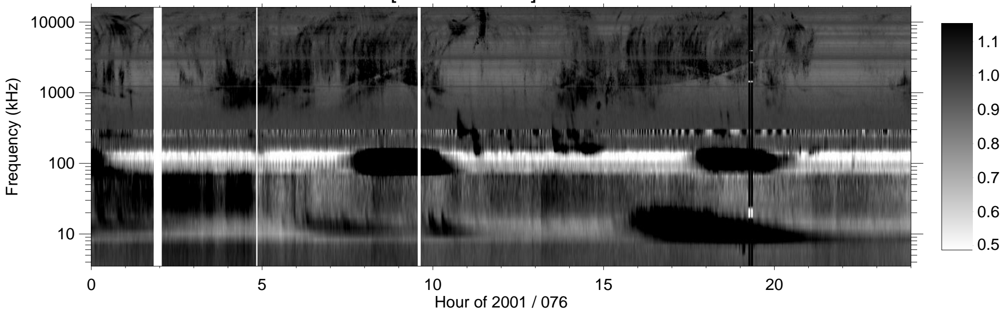
RPWS [ABCH1H2/Ex] (-B) 2001/03/17
