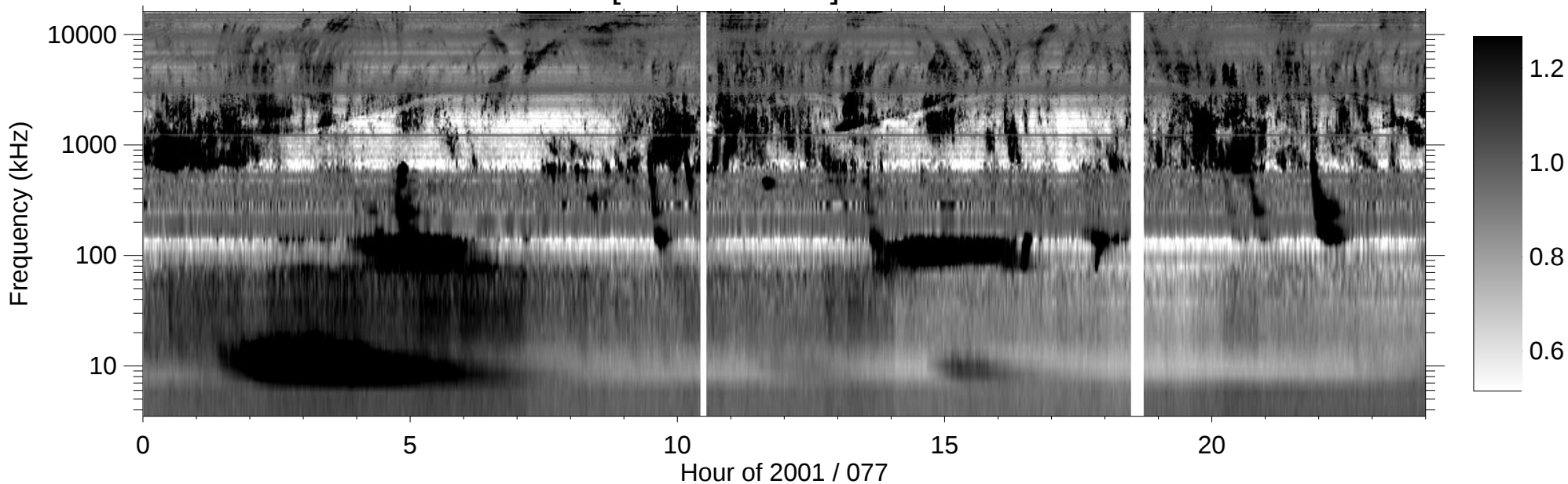
RPWS [ABCH1H2/Ex] (-B) 2001/03/18
