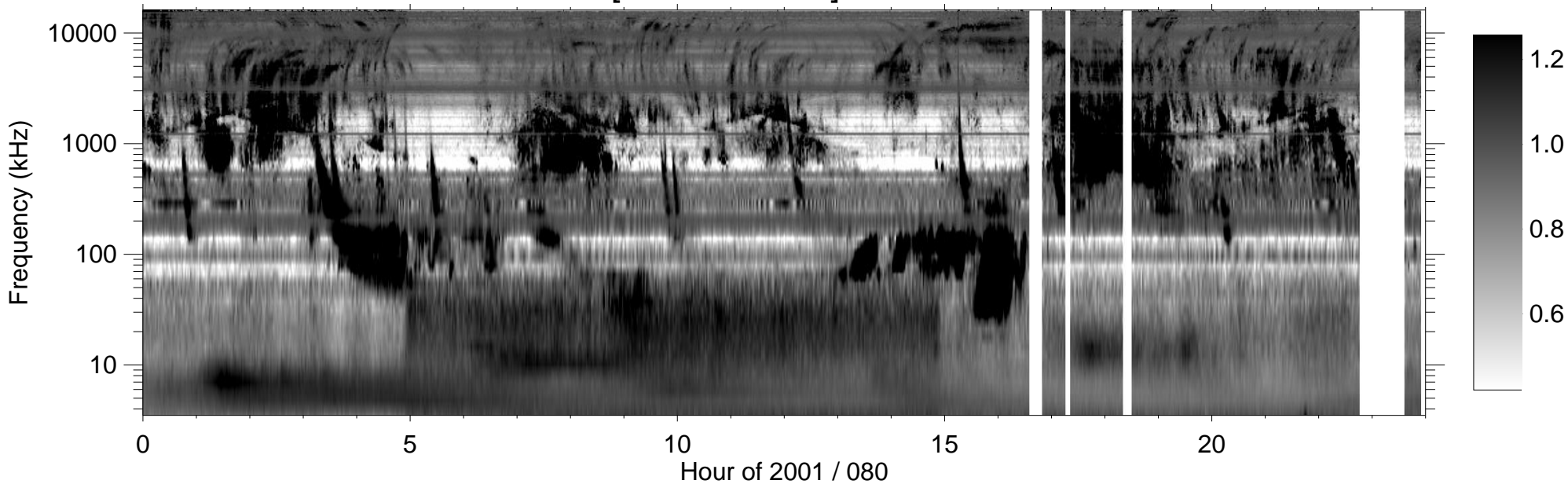
RPWS [ABCH1H2/Ex] (-B) 2001/03/21
