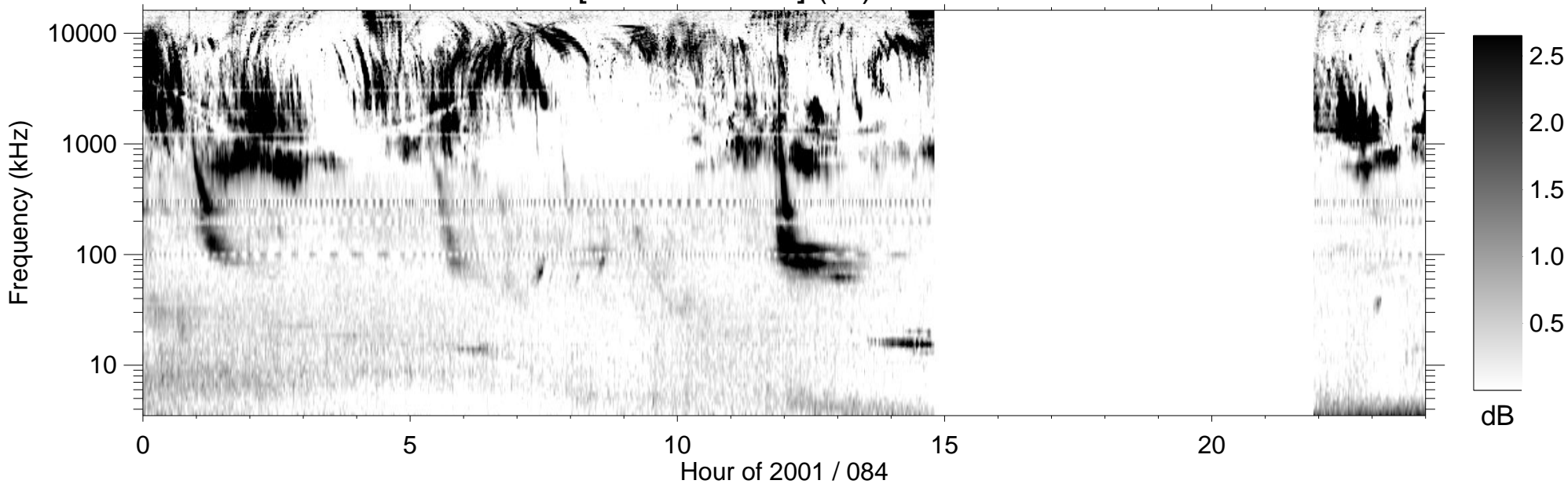
RPWS [ABCH1H2/Ex] (-B) 2001/03/25
