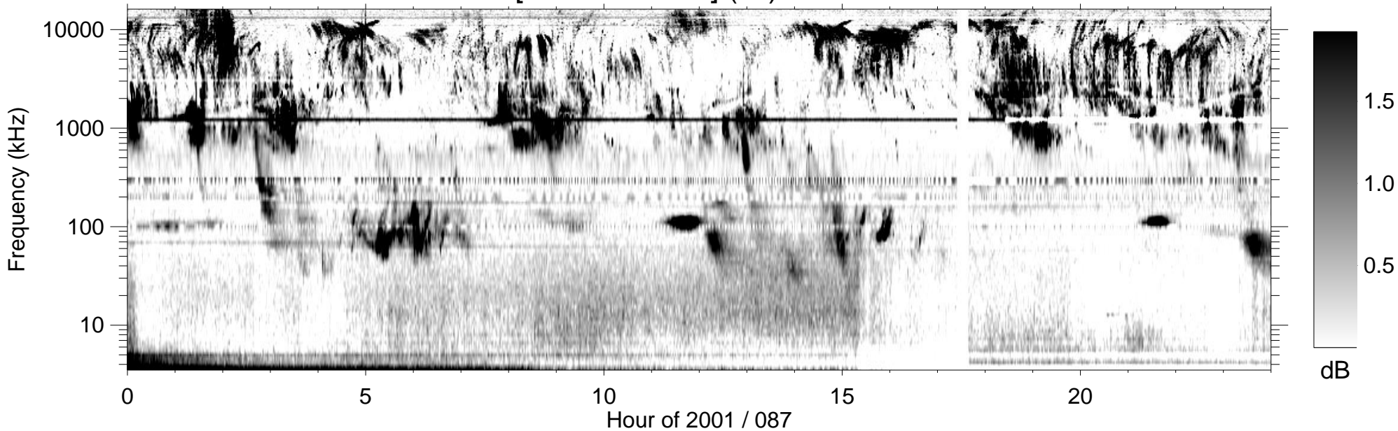
RPWS [ABCH1H2/Ex] (-B) 2001/03/28
