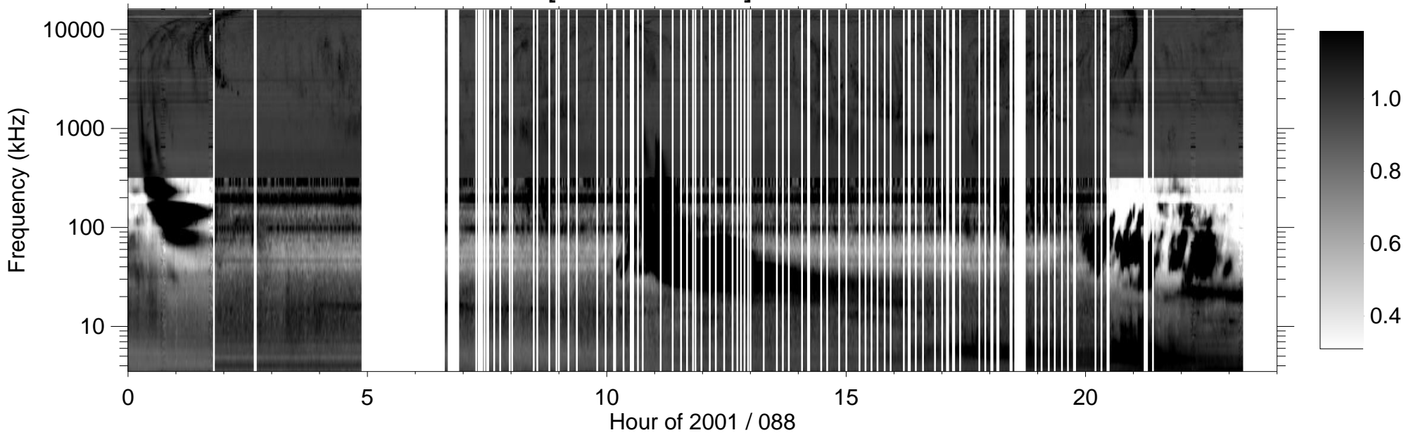
RPWS [ABCH1H2/Ex] (-B) 2001/03/29
