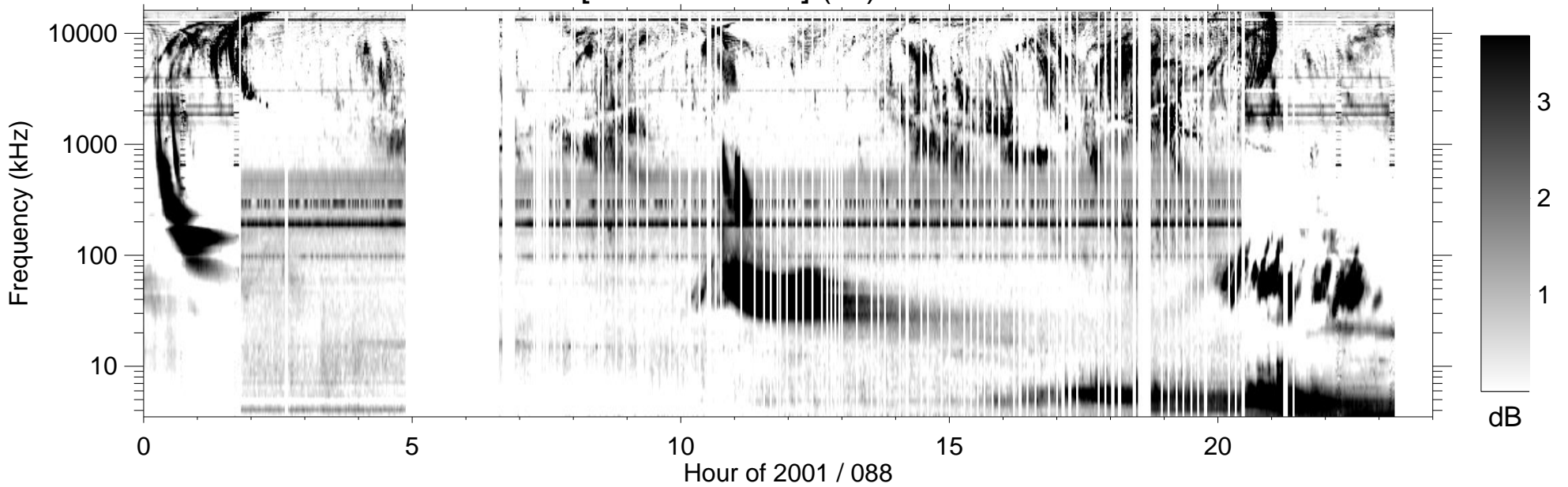
RPWS [ABCH1H2/Ex] (-B) 2001/03/29
