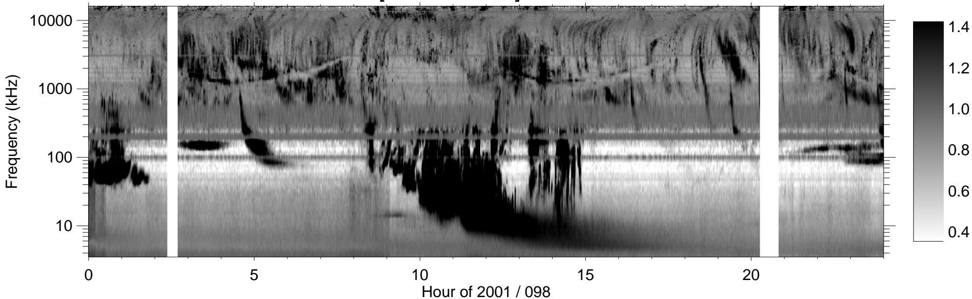
RPWS [ABCH1H2/Ex] (-B) 2001/04/08
