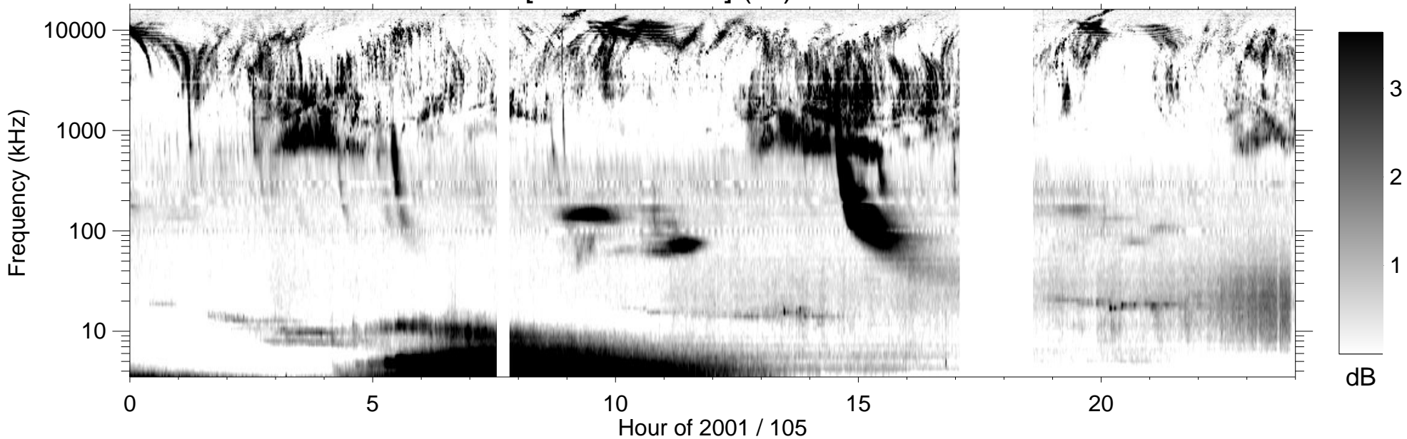
RPWS [ABCH1H2/Ex] (-B) 2001/04/15
