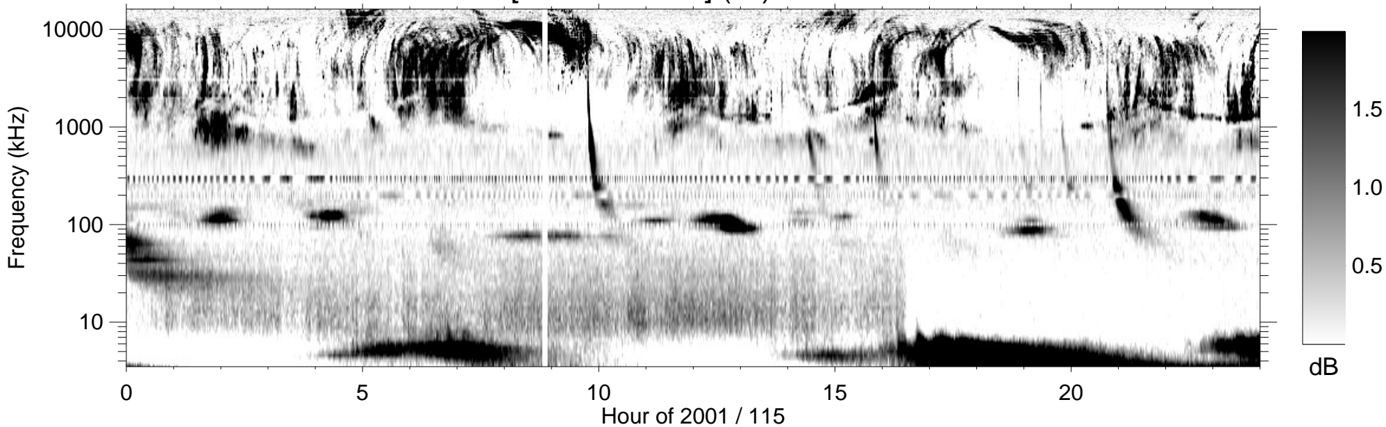
RPWS [ABCH1H2/Ex] (-B) 2001/04/25
