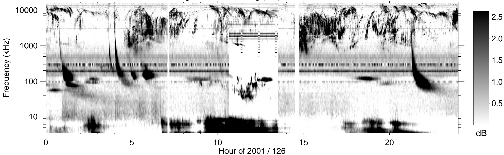
RPWS [ABCH1H2/Ex] (-B) 2001/05/06
