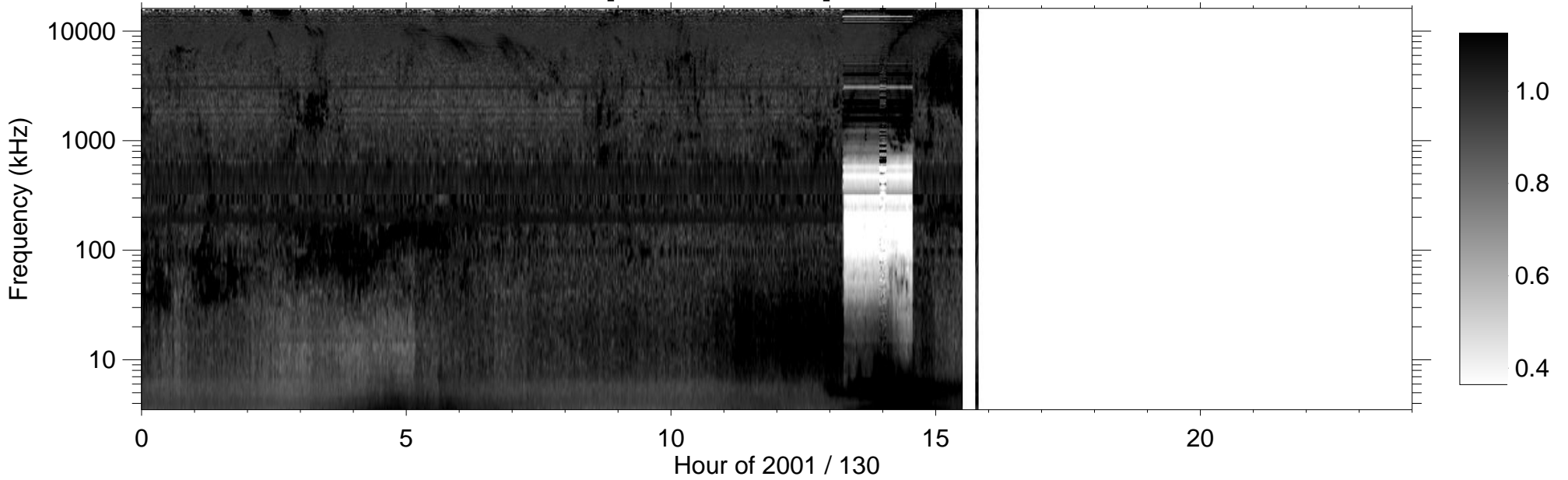
RPWS [ABCH1H2/Ex] (-B) 2001/05/10
