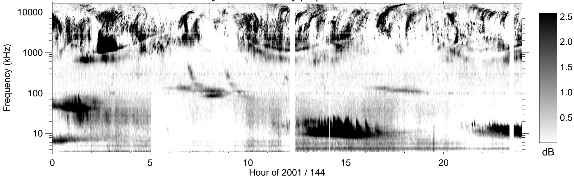
RPWS [ABCH1H2/Ex] (-B) 2001/05/24
