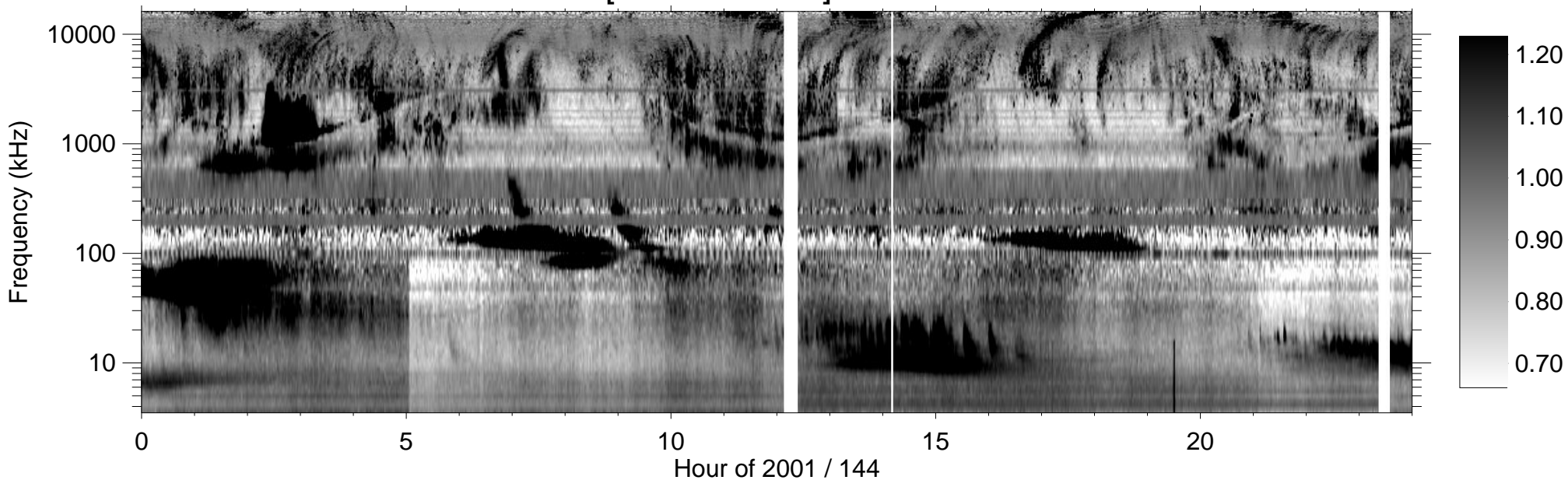
RPWS [ABCH1H2/Ex] (-B) 2001/05/24
