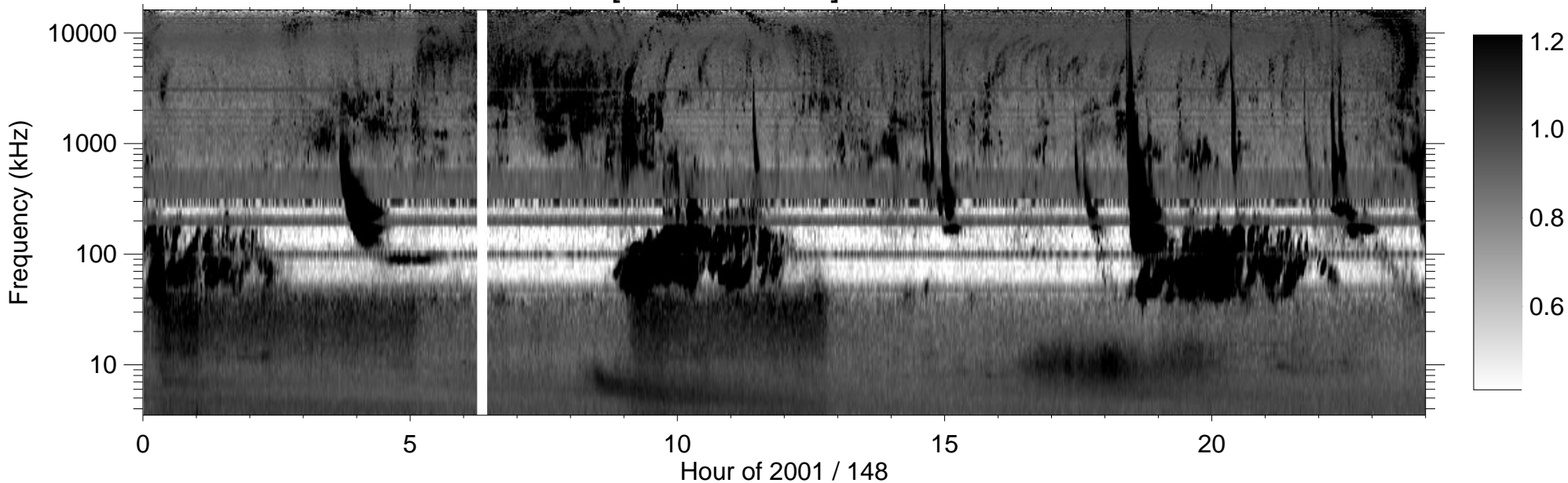
RPWS [ABCH1H2/Ex] (-B) 2001/05/28
