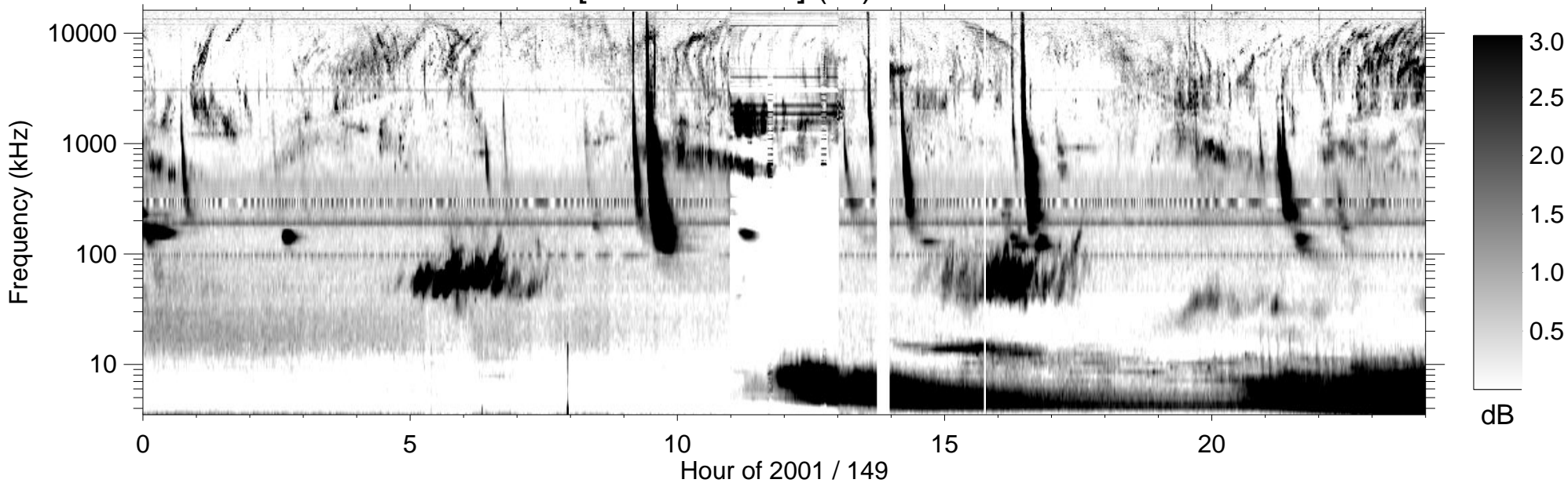
RPWS [ABCH1H2/Ex] (-B) 2001/05/29
