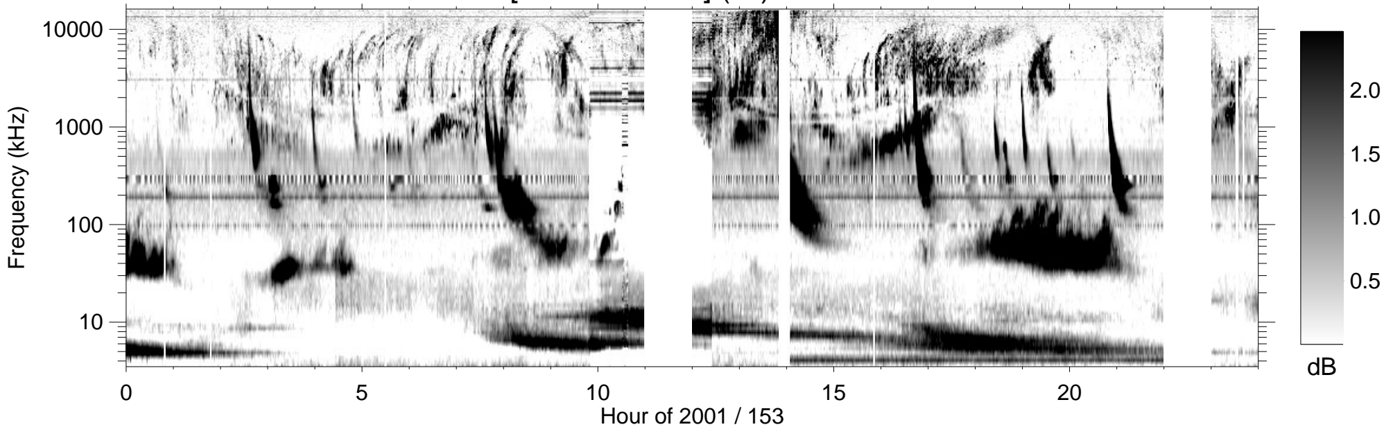
RPWS [ABCH1H2/Ex] (-B) 2001/06/02
