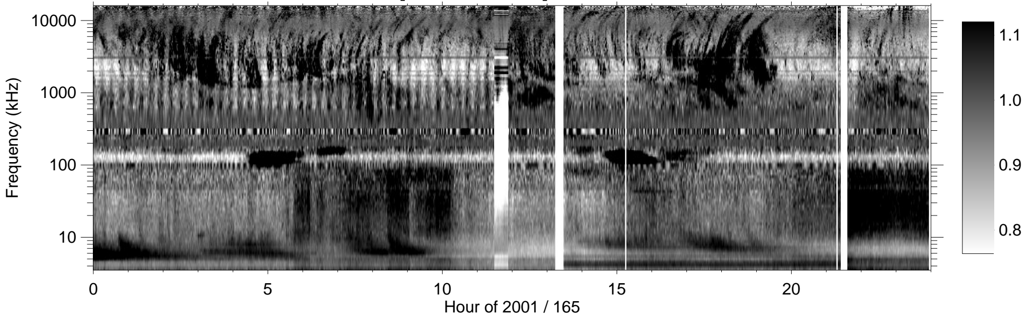
RPWS [ABCH1H2/Ex] (-B) 2001/06/14
