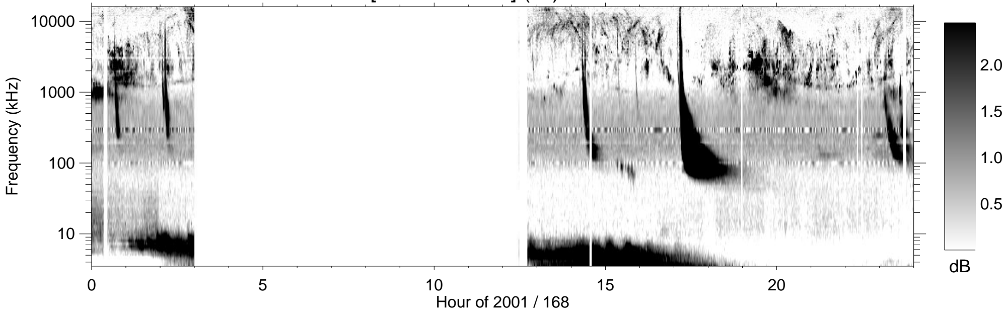
RPWS [ABCH1H2/Ex] (-B) 2001/06/17
