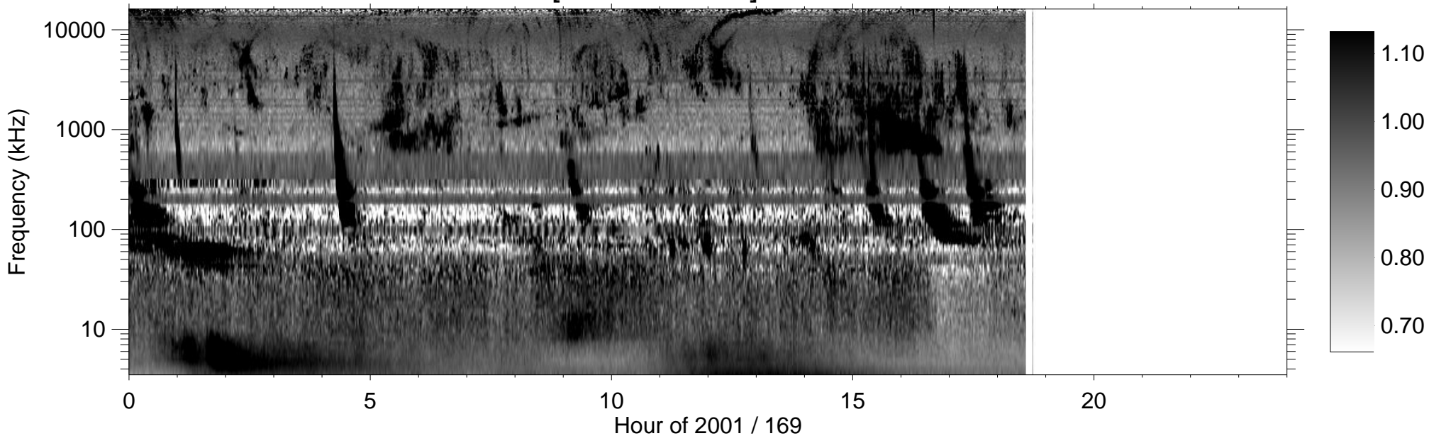
RPWS [ABCH1H2/Ex] (-B) 2001/06/18
