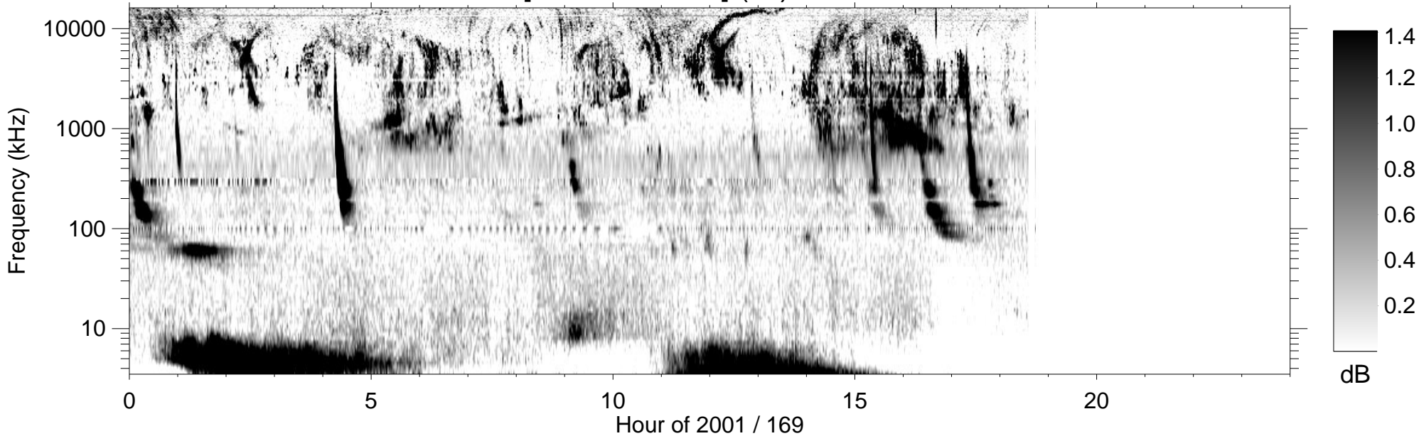
RPWS [ABCH1H2/Ex] (-B) 2001/06/18
