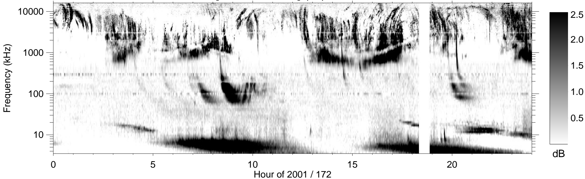
RPWS [ABCH1H2/Ex] (-B) 2001/06/21
